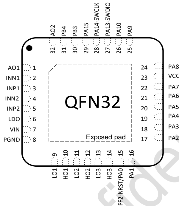
图 3-1 QFN32(4*4) Pinout1 PY32MD410K1xU
